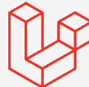
Laravel
